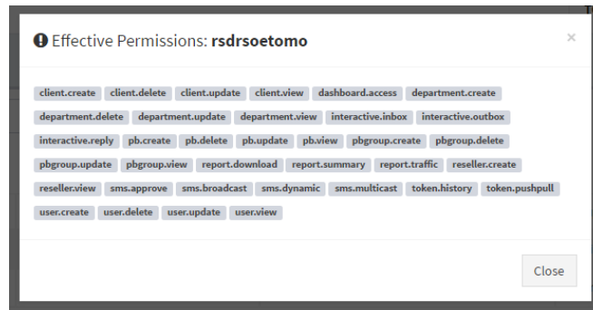
Gambar 10-2 Effective Permission Menu Users
